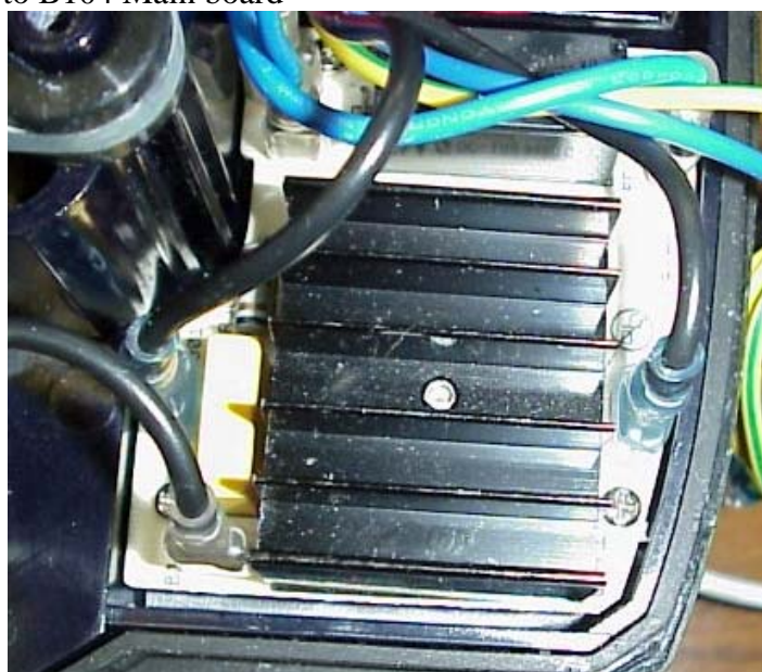
Figure 3: Relay/Rectifier board
