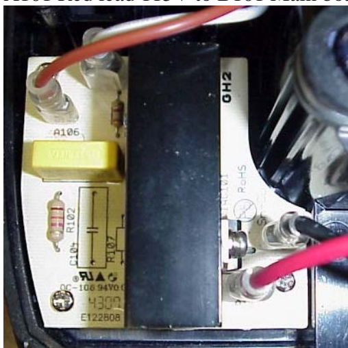
Figure 4: TRIAC board
