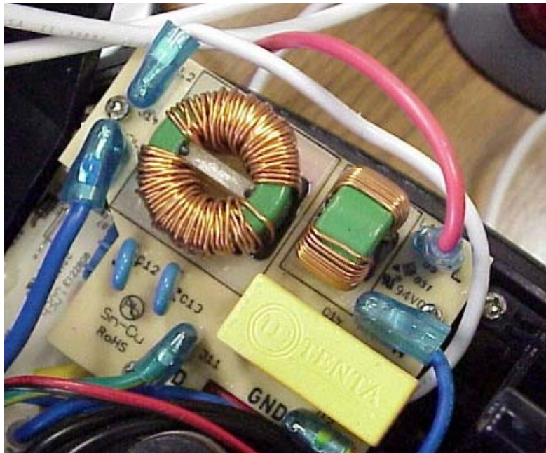
Figure 2. RFI Board
